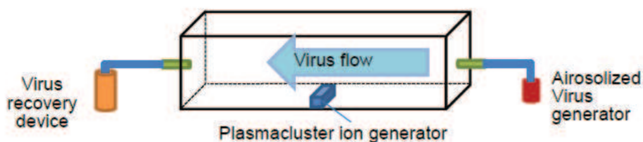
Figure 1 Test device diagram
